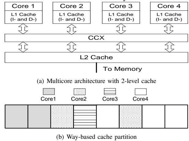
Fig. 1. Hardware model.
