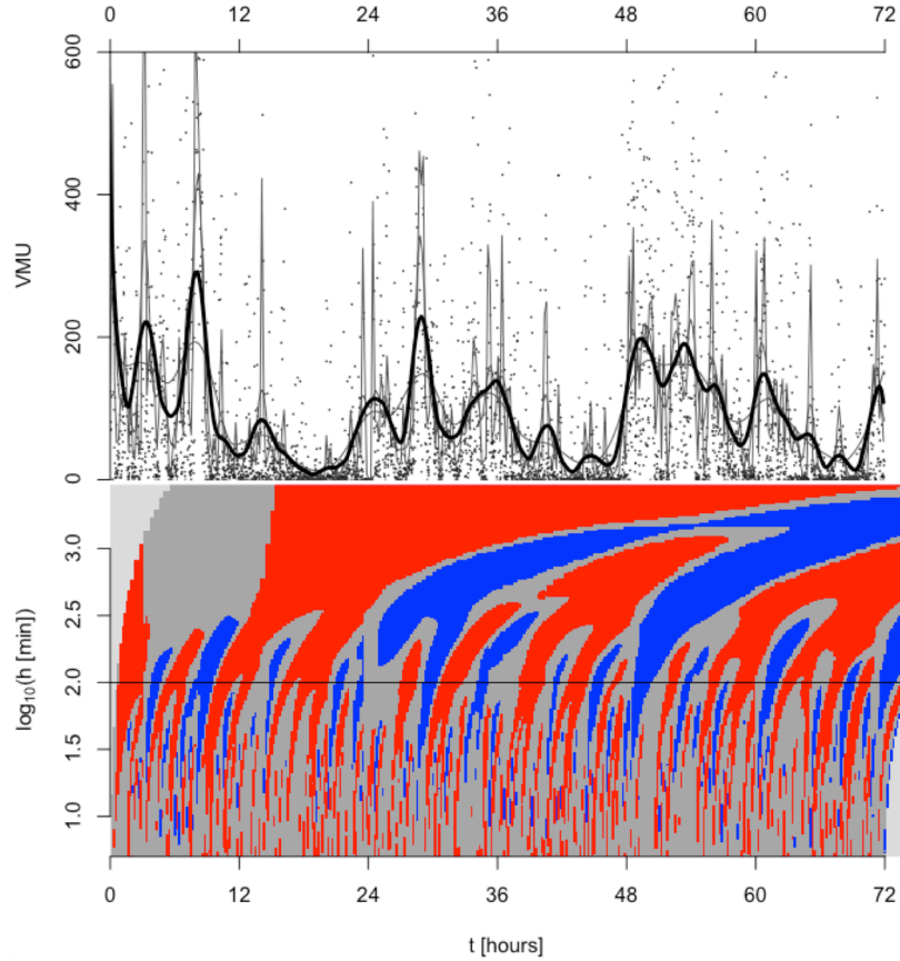
Figure 1: Upper panel: The sensor samplings for each minute in three days for a COPD patient as dots overlaid by a family plot of kernel smooths with four different bandwidths; h = \{10, 50, 100, 200\} min with h = 100 min highlighted. For clarity, the upper limit of the y-axis is cropped such that some data points are not shown. Lower panel: The c-SiZer plot with statistically significant changes color coded as red decreasing and blue increasing activity level. The highlighted bandwidth in the upper panel is indicated by the horizontal line. Light gray areas in the upper left and lower right corners are where the effective sample size is too small for a normality assumption to hold, and dark gray areas have no significant gradient.
