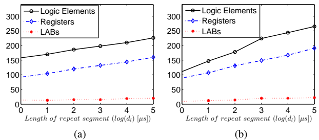
Fig. 10.: Resource usage with increasing busy-window period. (a) Dynamic counters monitoring; (b) l -repetitive monitoring.
